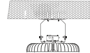
Surface Mounted
