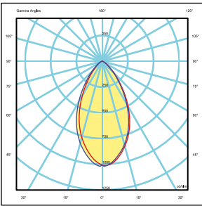
Photometry T60
