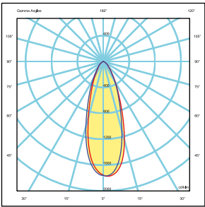
Photometry T25
